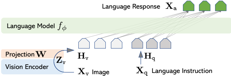
Figure 1: LLaVA network architecture.
